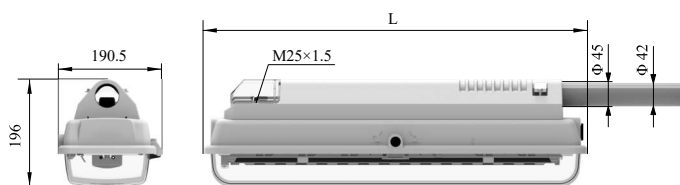
Z.186□/2□1P Full plastic explosion-proof LED linear light fittings(Pole Mounting)
