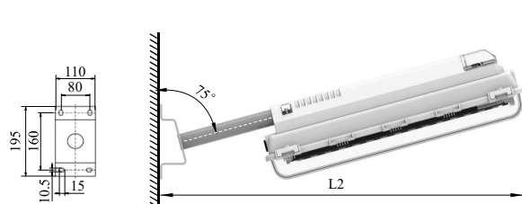
D8739 Wall mounting bracket of pole type
