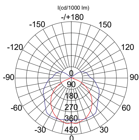
type Z0865 - 2 x 18 Watt
