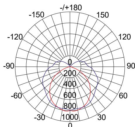
type Z0866 - 2 x 36 Watt
